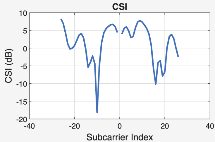
Channel Estimate, BER=0
